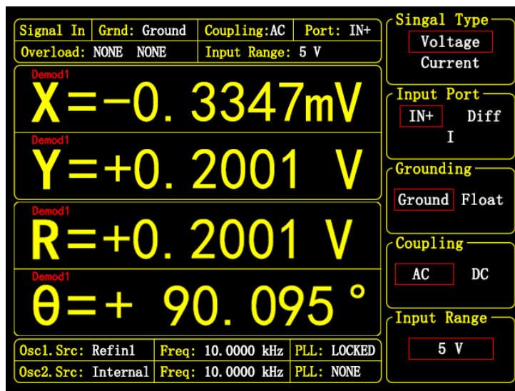
图 40. [INPUT/FILTERS] 子菜单
