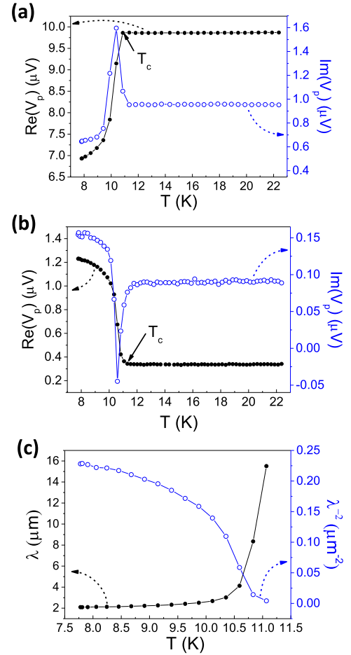
FIG. 5. Mutual inductance measurement results from (a) transmission-type and (b) reflection-type configurations. (c) Magnetic penetration depth \lambda and superfluid density n_s \propto \lambda^{-2} extracted from the reflection-type measurement results. The curved arrows indicate the Y axis location corresponding to each data set.
